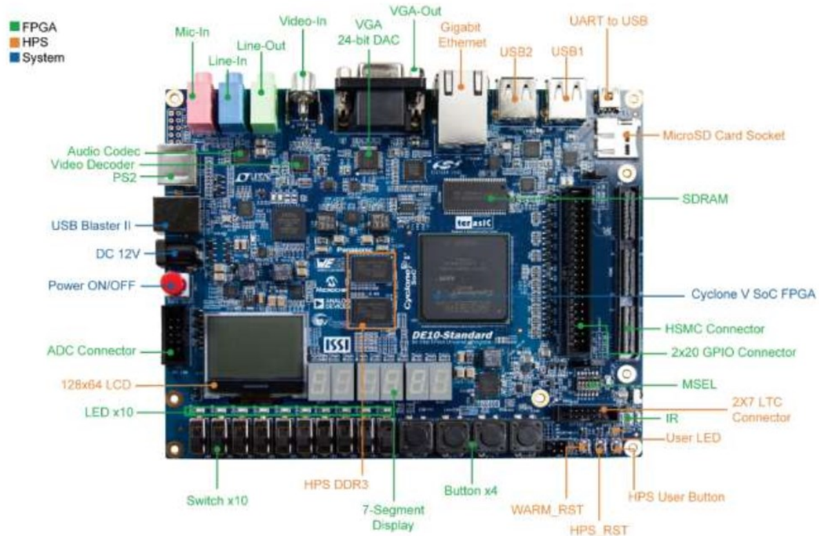
Figure 2-1 DE10-Standard development board (top view)
